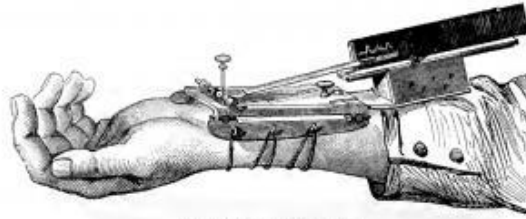
Fig. 106. Sphygmograph direct.
